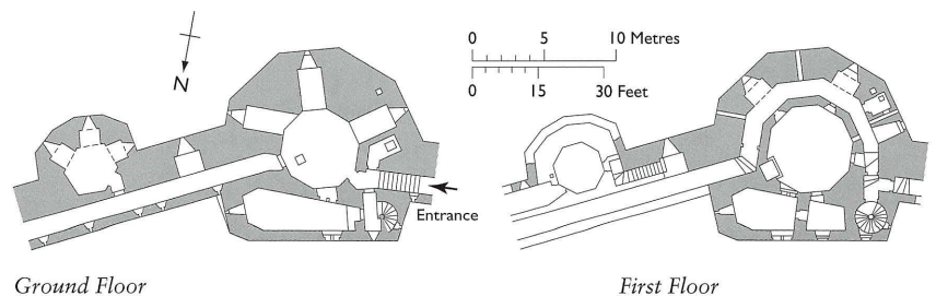
Below: Black Tower (right) and Cistern Tower (left) floor plans.
