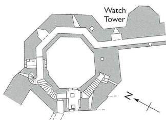
Mezzanine showing wall-passages
